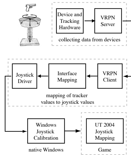
Figure 3. The ChairIO Interface Architecture.
